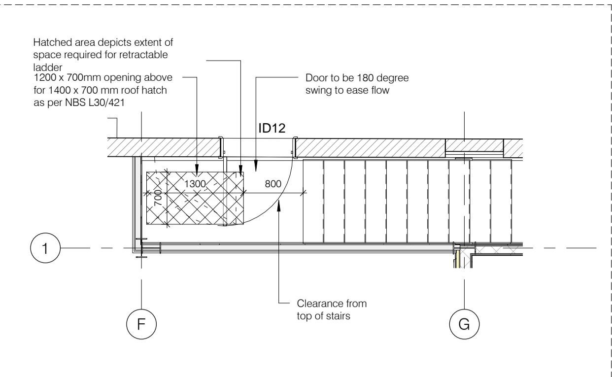
2 Emergency Exit Stairwell 1 : 50
